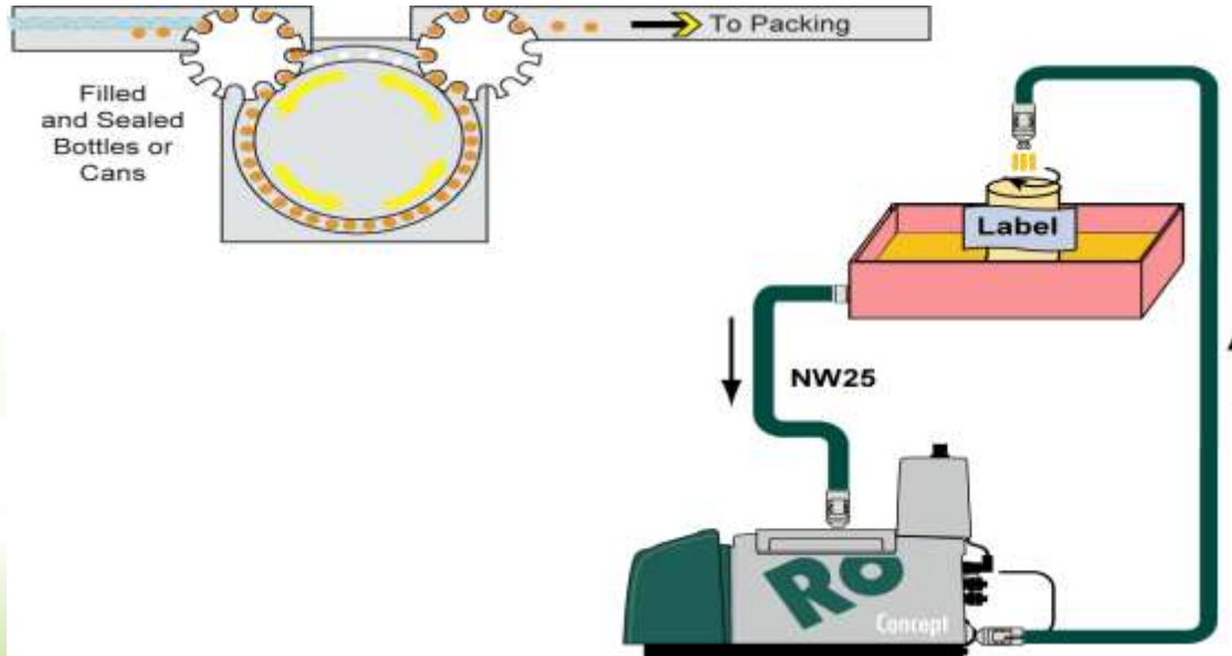
Labelling Process – Pot Filling
